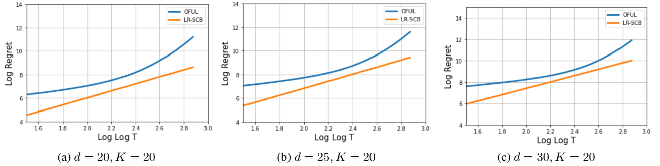
Figure 3. Scaling of \log R(T) with respect to \log \log T for OFUL and LR-SCB. The linear increase of LR-SCB indicates a \text{polylog}(T) regret. The plots are produced by taking an average over 50 trials.
