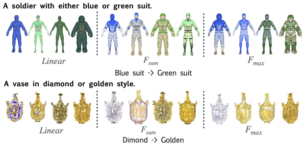
Figure 7. Results on Text2Mesh generation from F_{\text{sum}} , F_{\text{max}} and linear combination ( \alpha = 0.5 ). See supplementary materials for a detailed description video.
