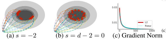
Figure 1. Results on a 2D ( d = 2 ) toy example with F_{\text{sum}} . We test two different choices of s in Riesz energy, including s = -2 (variance) and s = d - 2 = 0 (logarithm energy). We can see that the logarithm energy yields more uniformly distributed points.
