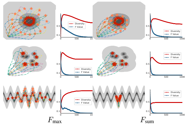
Figure 3. Results on toy examples with F_{\text{max}} and F_{\text{sum}} . The red and orange stars show the 1000th-iteration and 200th-iteration results. The curve shows the value of the target function and diversity term during optimization.
