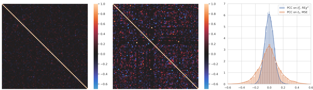
Figure 5. Heatmaps and distributions of the PCCs between different elements of embedding vectors. The left subfigure is the heatmap for the proposed method (CNN-ED-5: \ell_2^2 : RE\chi^2 ). The middle subfigure is the heatmap for the comparative/ablation experiment (CNN-ED-5: \ell_2 : MSE). The right subfigure is for the histograms of the PCCs for the two models (diagonal 1s are omitted).
