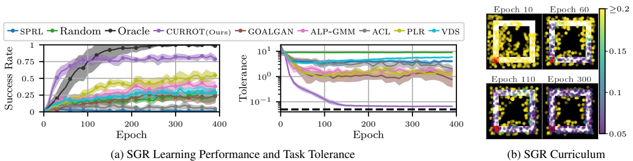
Figure 4. a) Left: Success rate on the feasible subspace of \mathcal{C} over learning epochs for different CRL methods in the sparse goal reaching (SGR) task. We also include a uniform sampling baseline (referred to as Random) as well as an oracle baseline which only samples the feasible tasks in the context space \mathcal{C} . Right: Median tolerance of tasks generated by different CRL methods as well as the uniform and oracle baseline. For both plots, mean and standard error are computed from 10 runs. b) Context distributions \hat{p}_{\mathcal{W}}(\mathbf{c}) for a run of CURROT on the sparse goal reaching task for epochs 10, 60, 110 and 300. The area in which the agent starts each episode is highlighted in red. Walls are shown in black. The position of the samples encodes the goal to be reached while the color encodes the tolerance with which the goal needs to be reached.
