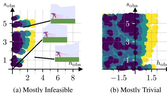
Figure 8. Sampling distribution \hat{p}_{\mathcal{W}}(\mathbf{c}) of CURROT on the bipedal walker stump track environment in the no expert knowledge setting in task spaces with (a) mostly infeasible and (b) mostly trivial tasks. Brighter colors indicate samples that correspond to later epochs of agent training. The small image visualize the obstacles that are encoded by the corresponding contexts. For environment details, please see (Romac et al., 2021).
