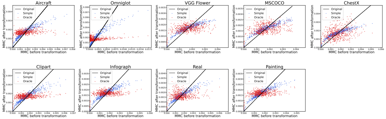
Figure 10. The Visualization of MMC of the other nine datasets before and after the use of simple and oracle transformation. All notations are the same as in Figure 6.
