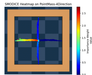
Figure 7. SMODICE weights.
