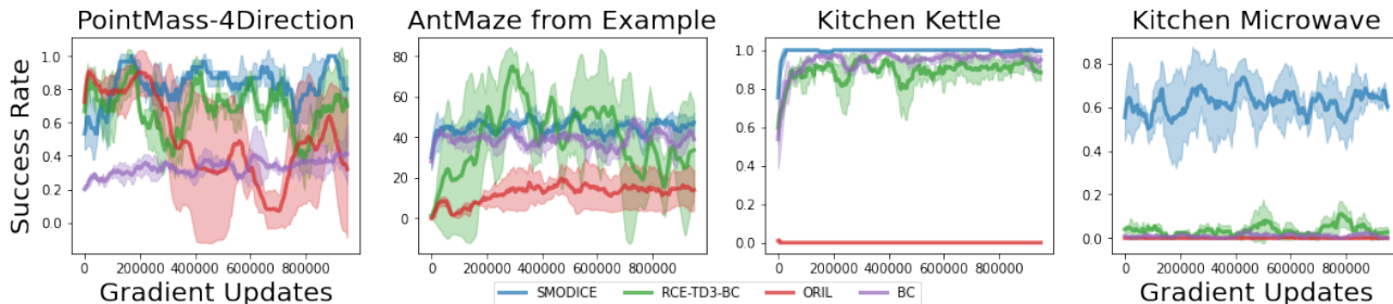
Figure 6. Offline imitation learning from examples results.
