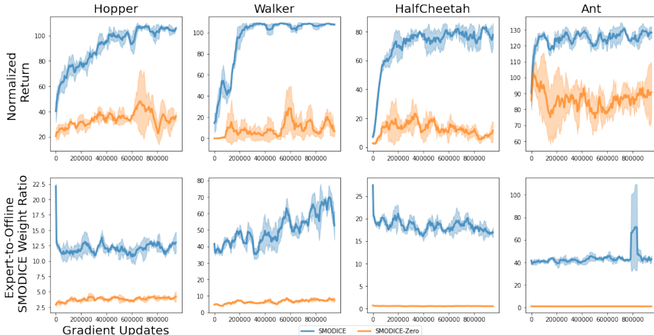
Figure 9. SMODICE vs. SMODICE-Zero. Using the discriminator-based reward, SMODICE assigns much higher weights to expert-quality data.
