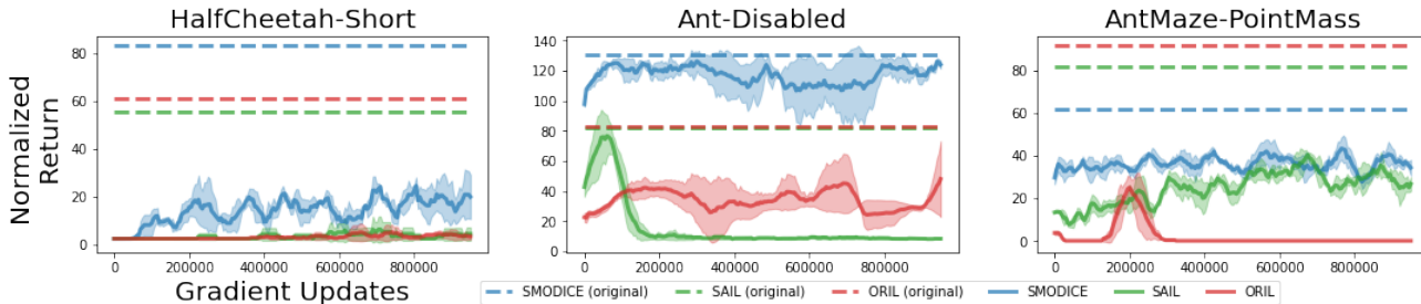
Figure 5. Offline imitation learning from mismatched experts results.
