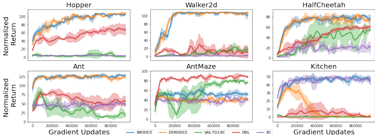
Figure 4. Offline imitation learning from observations results.
