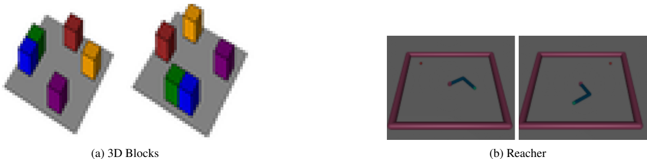
Figure 12: Original observations and their G -transformed versions
