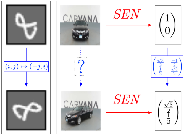
Figure 1: Equivariant networks consider transformations of inputs that are easy to compute, such as in-plane rotations for MNIST digits. This paper considers transformations that are difficult to compute, such as rotations of 3D objects like cars (Carvana, 2017). Symmetric embedding networks learn representations which are transformed simply.
