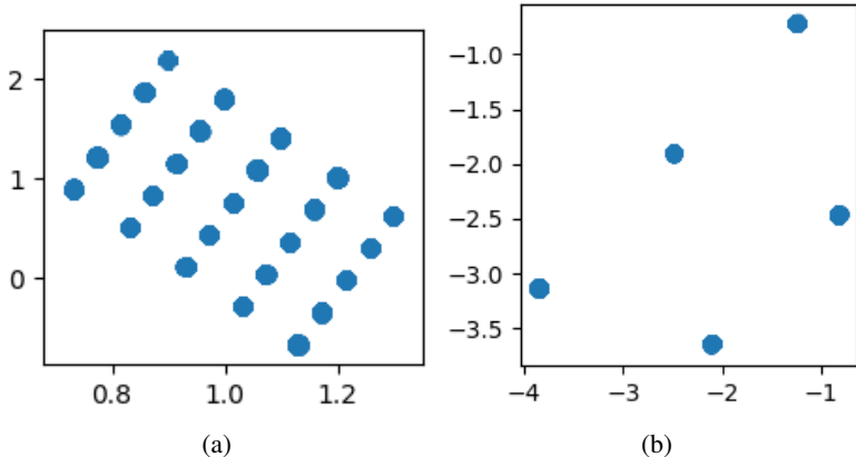
Figure 8: 2D Shapes: learned embeddings for all states in the evaluation set when trained on only the up action. Our model (left) is able to generalize well and learns the correct underlying 5 \times 5 grid. The non-equivariant model (right) learns a degenerate solution
