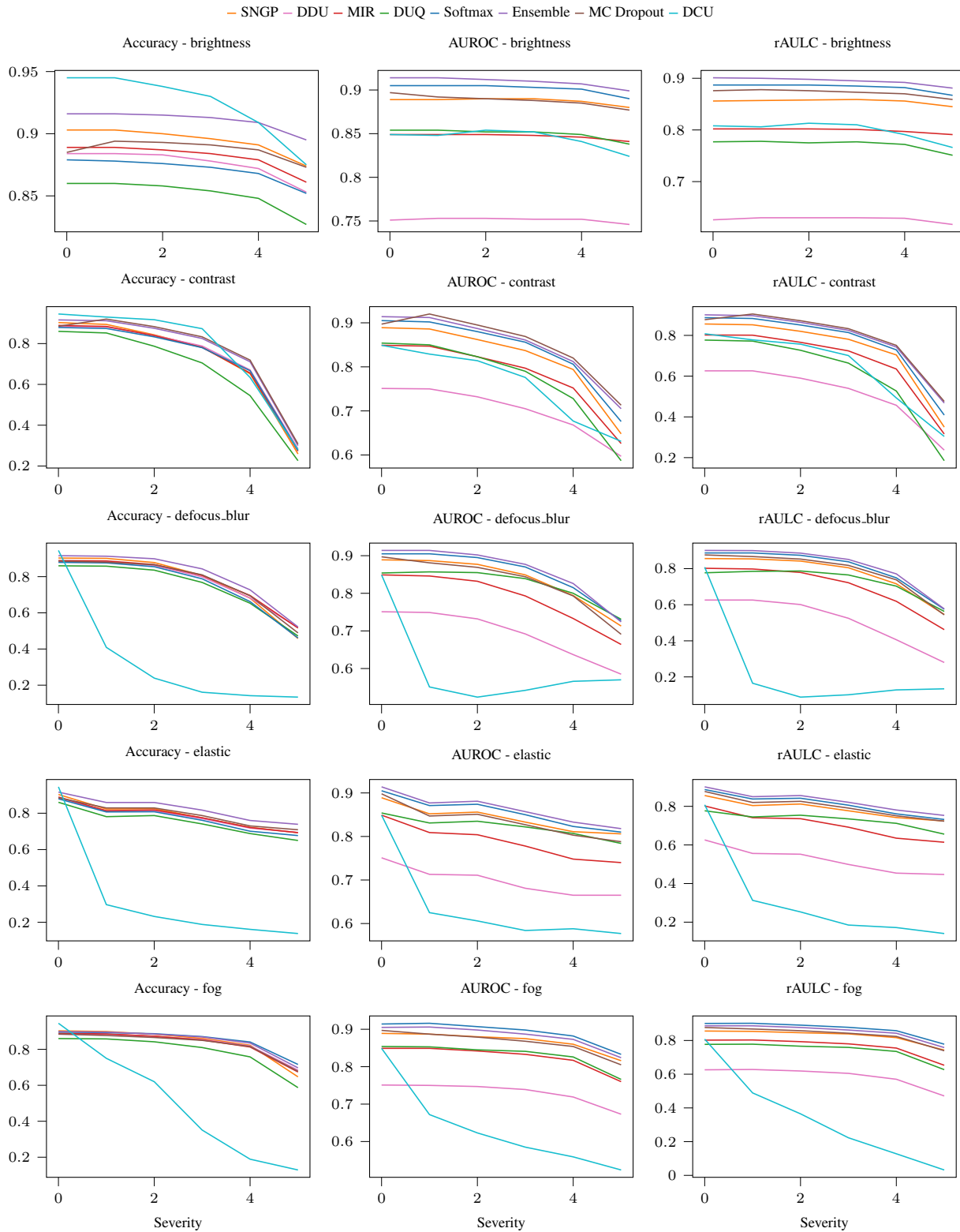
Figure 9. We here compare the performance of DUMs and of the baselines under different corruption types and severities applied on the CIFAR10-C dataset. We show the accuracy, AUROC and rAULC (vertical axis) for each method depending on the corruption severity (horizontal axis) of the following corruption types (listed from top to bottom): brightness, contrast, defocus blur, elastic, fog.
