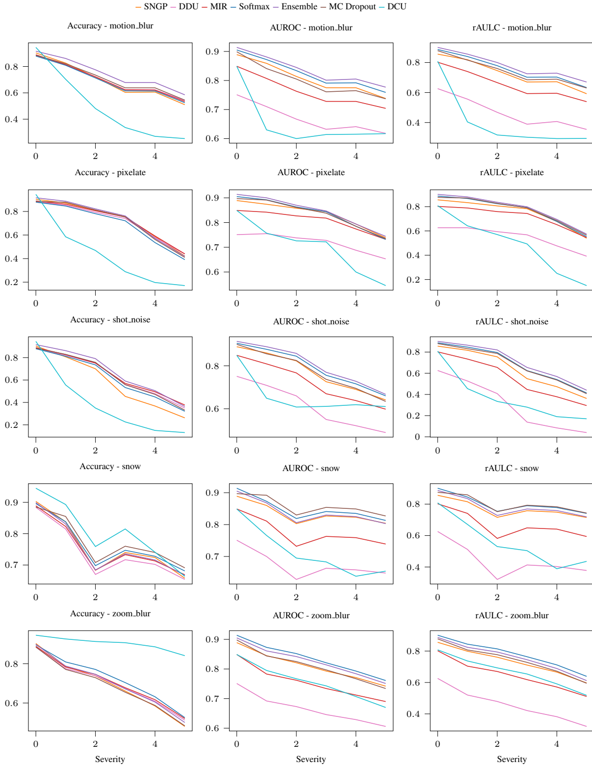
Figure 14. We here compare the performance of DUMs and of the baselines under different corruption types and severities applied on the CIFAR100-C dataset. We show the accuracy, AUROC and rAUC (vertical axis) for each method depending on the corruption severity (horizontal axis) of the following corruption types (listed from top to bottom): motion blur, pixelate, shot noise, snow, zoom blur.
