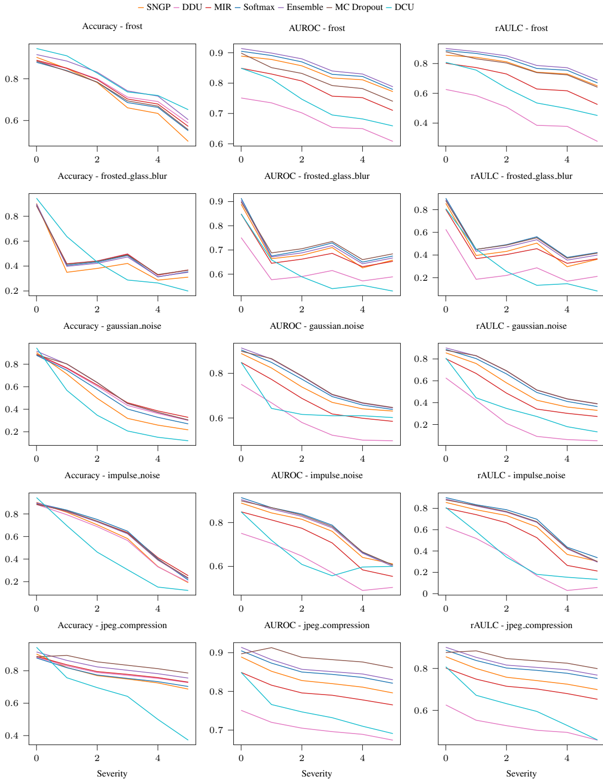
Figure 13. We here compare the performance of DUMs and of the baselines under different corruption types and severities applied on the CIFAR100-C dataset. We show the accuracy, AUROC and rAULC (vertical axis) for each method depending on the corruption severity (horizontal axis) of the following corruption types (listed from top to bottom): frost, frosted glass blur, gaussian noise, impulse noise, jpeg compression.
