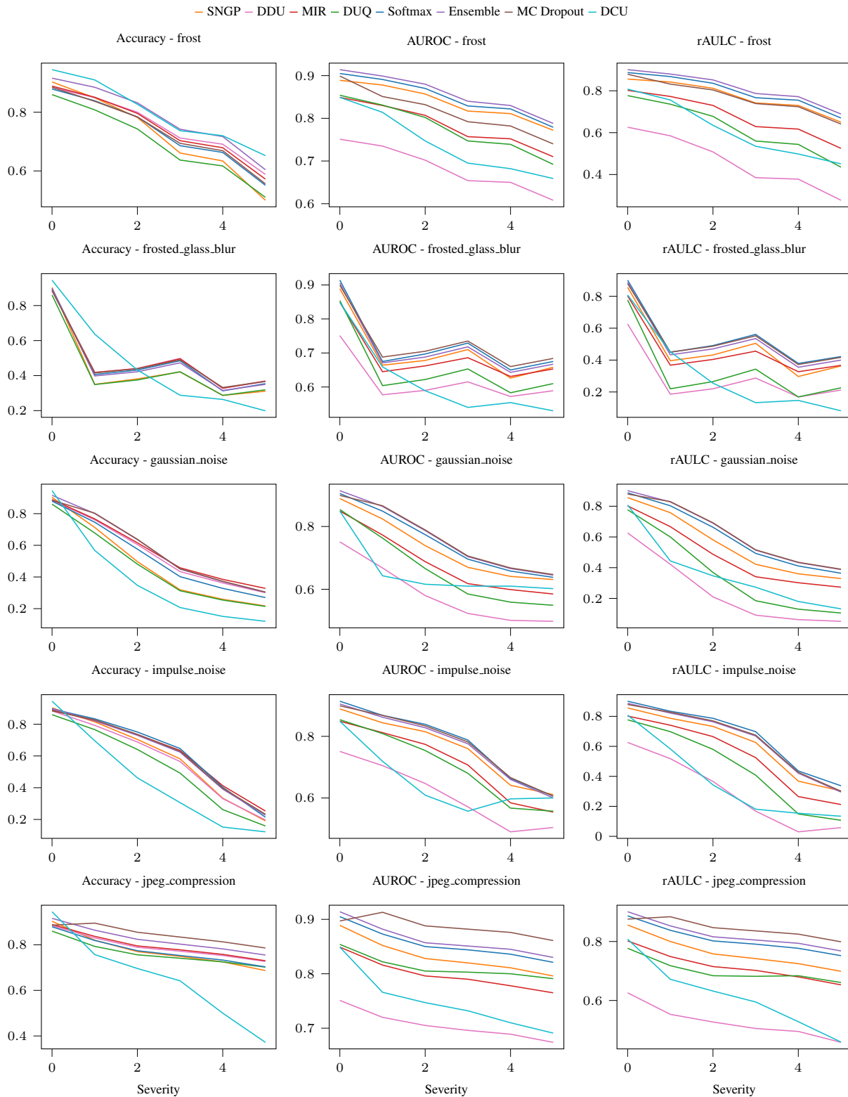
Figure 10. We here compare the performance of DUMs and of the baselines under different corruption types and severities applied on the CIFAR10-C dataset. We show the accuracy, AUROC and rAULC (vertical axis) for each method depending on the corruption severity (horizontal axis) of the following corruption types (listed from top to bottom): frost, frosted glass blur, gaussian noise, impulse noise, jpeg compression.
