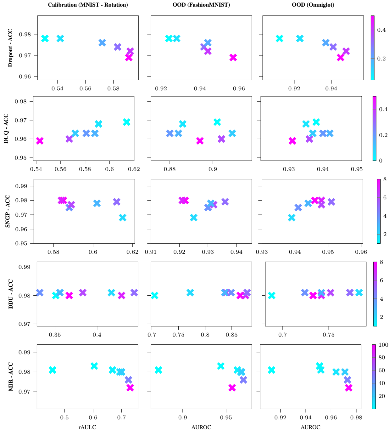
Figure 4. Trained on MNIST. Vertical axis: Test accuracy. Horizontal axis: rAULC (left), AUROC against FashionMNIST (center) and Omniglot (right) for Dropout (1st row), DUQ (2nd row), SNGP (3rd row), DDU (4th row) and MIR (5th row) using different regularization strength. For SNGP a larger hyperparameter corresponds to less regularization. For Dropout and MIR we observe a correlation between regularization strength and performance.
