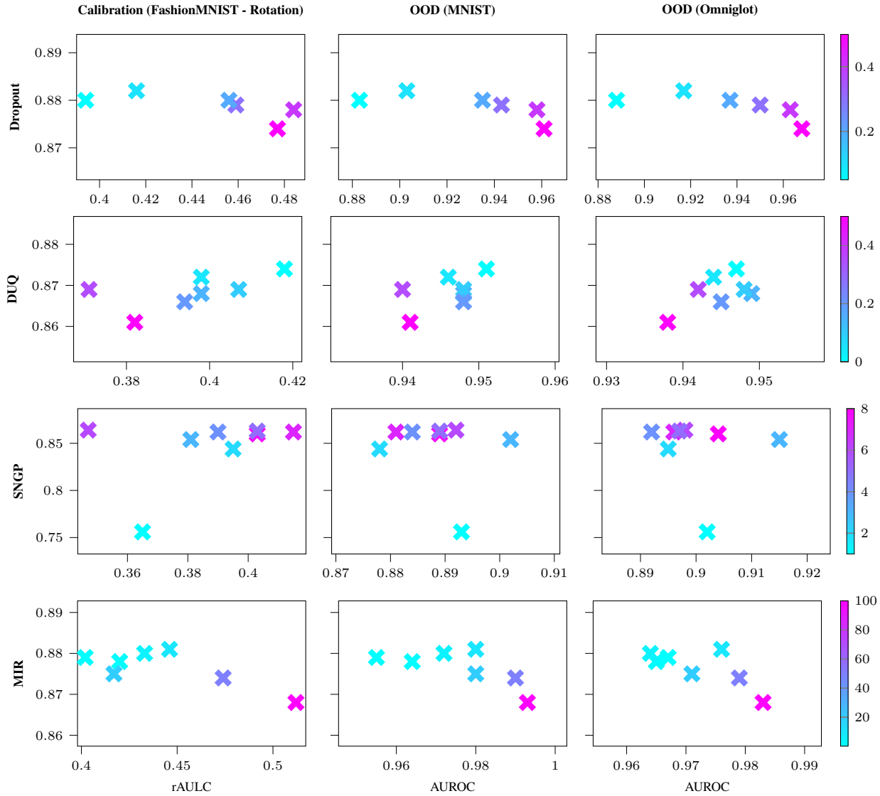
Figure 5. Trained on FashionMNIST. Vertical axis: Test accuracy. Horizontal axis: rAULC (left), AUROC against MNIST (center) and Omniglot (right) for Dropout (1st row), DUQ (2nd row), SNGP (3rd row) and MIR (4th row) using different regularization strength. For SNGP a larger hyperparameter corresponds to less regularization. For Dropout and MIR we observe a correlation between regularization strength and performance.
