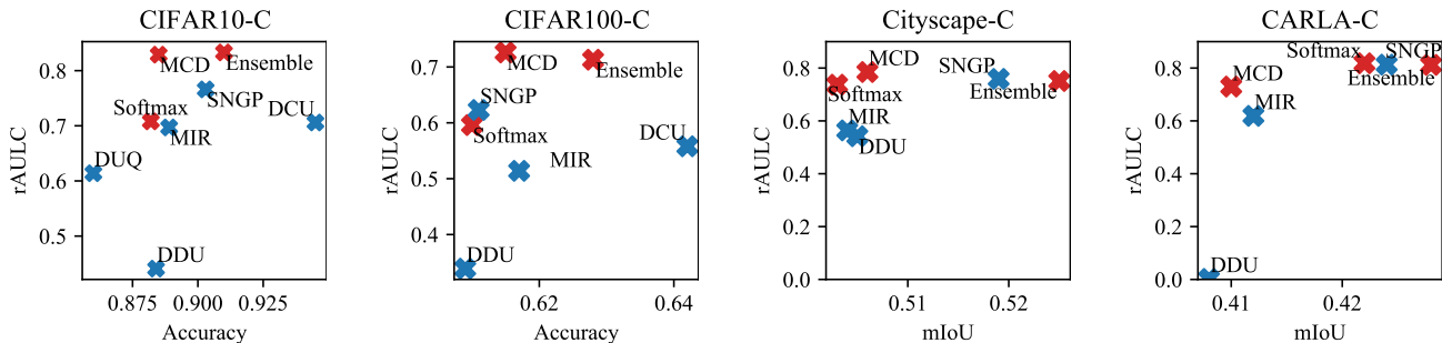
Figure 3. Scatter plots for Accuracy/mIoU versus rAULC on 4 testsets, based on Tab. 2 and 4. The baselines (red) usually occupy the top part of the figure, confirming their effectiveness of uncertainty calibration. Among the DUMs (blue), SNGP and MIR are closer to the region of baselines than others. For realistic shifts (CARLA-C), a significant drop of uncertainty calibration performance can be found for DDU. (“MCD”=“MC Dropout”)
