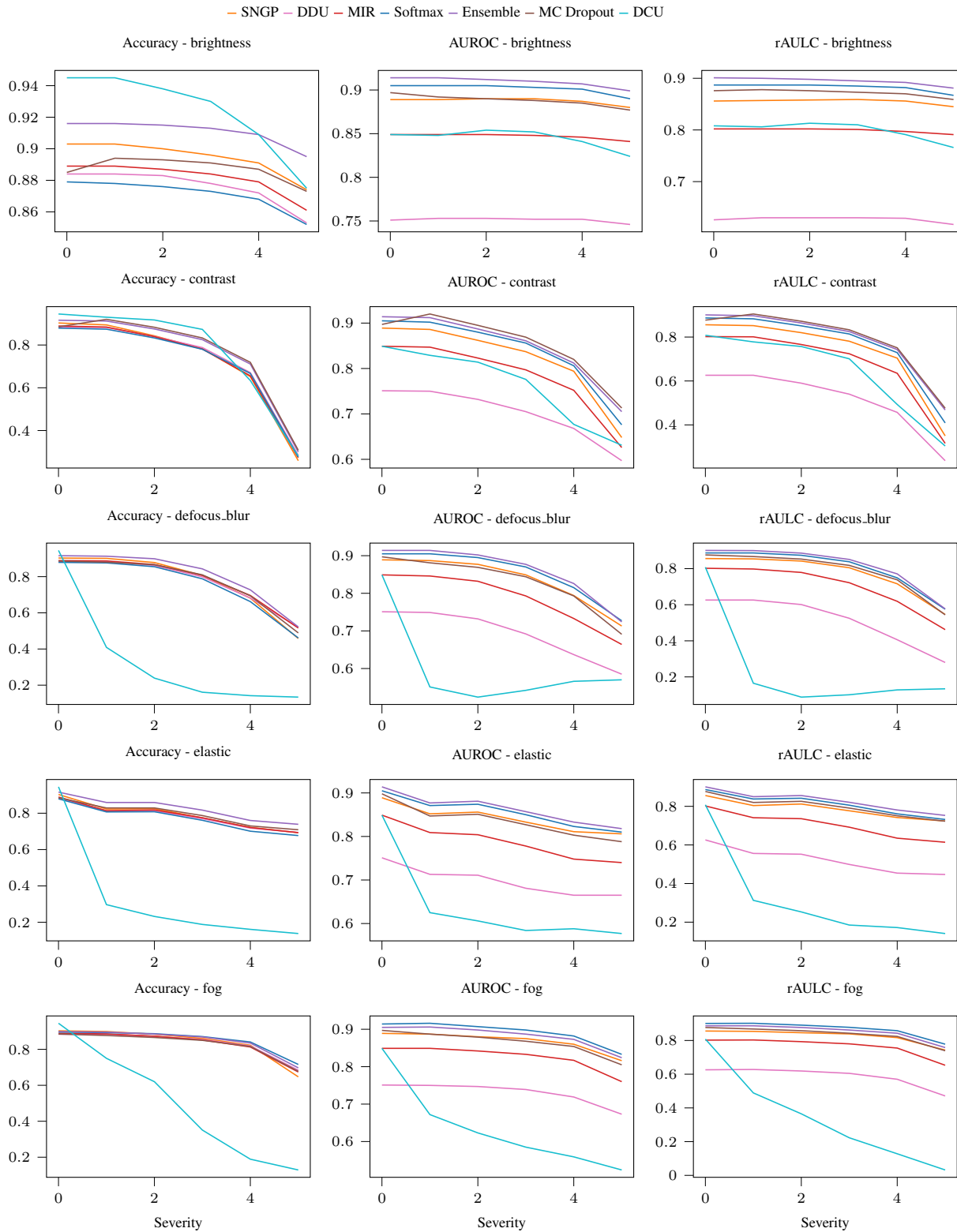
Figure 12. We here compare the performance of DUMs and of the baselines under different corruption types and severities applied on the CIFAR100-C dataset. We show the accuracy, AUROC and rAULC (vertical axis) for each method depending on the corruption severity (horizontal axis) of the following corruption types (listed from top to bottom): brightness, contrast, defocus blur, elastic, fog.
