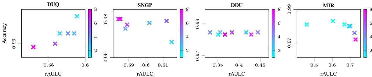
Figure 2. We analyze the sensitivity of DUQ (Van Amersfoort et al., 2020), SNGP (Liu et al., 2020), MIR (Postels et al., 2020) and DDU (Mukhoti et al., 2021) to their regularization strength. Therefore, we train models on MNIST and evaluate on continuously shifted data by rotating from 0 to 180 degrees in steps of 20 degrees. We plot the accuracy on the unperturbed testset against the rAULC computed using data from all levels of perturbation. Only for MIR we observe a clear, positive correlation between regularization strength and calibration. For DDU and SNGP, smaller regularization parameter denotes stronger regularization.
