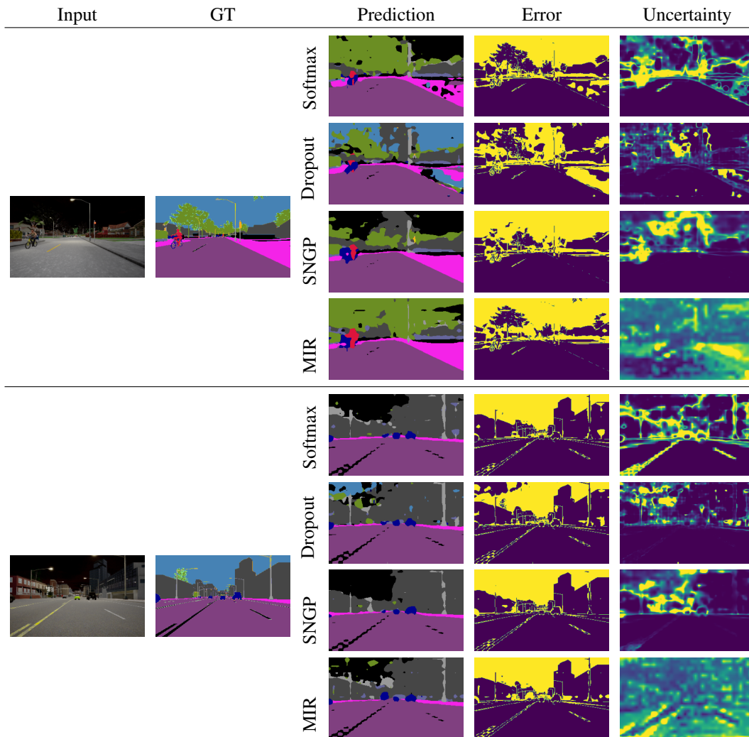
Figure 7. Qualitative comparison of uncertainty from Softmax, MC Dropout, SNGP and MIR under maximal time-of-the-day distribution shift ( i.e. Azimuth angle of the sun = -5^\circ ). We show the input image (Input) and the ground truth mask (GT), and we report for each method the predicted segmentation mask (Prediction), the error mask (Error) and the uncertainty mask (Uncertainty).
