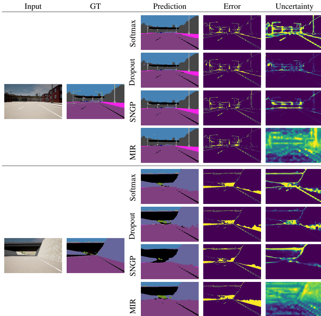
Figure 6. Qualitative comparison of uncertainty from Softmax, MC Dropout, SNGP and MIR under minimal time-of-the-day distribution shift ( i.e. Azimuth angle of the sun = 85^\circ ). We show the input image (Input) and the ground truth mask (GT), and we report for each method the predicted segmentation mask (Prediction), the error mask (Error) and the uncertainty mask (Uncertainty).
