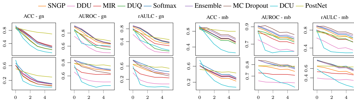
Figure 1. Softmax entropy, ensembles (Lakshminarayanan et al., 2017), MC dropout (Gal & Ghahramani, 2016), DUQ (Van Amersfoort et al., 2020), SNGP (Liu et al., 2020), MIR (Postels et al., 2020), DDU (Mukhoti et al., 2021) and DCU (Winkens et al., 2020) on CIFAR10-C (upper row) and CIFAR100-C (lower row) (Hendrycks & Dietterich, 2019). We show the accuracy, AUROC and rAULC on the corruptions gaussian_noise (gn) and motion_blur (mb) against the corruption severity. While all methods, except DCU, demonstrate a similar accuracy, DUMs - in particular methods based on generative modeling of hidden representations - yield worse calibration. DUQ did not converge on CIFAR100. Other corruptions are included in the supplement.
