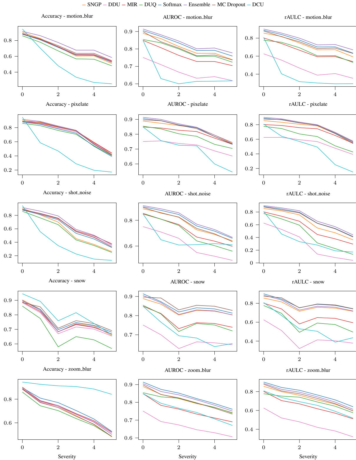
Figure 11. We here compare the performance of DUMs and of the baselines under different corruption types and severities applied on the CIFAR10-C dataset. We show the accuracy, AUROC and rAULC (vertical axis) for each method depending on the corruption severity (horizontal axis) of the following corruption types (listed from top to bottom): motion blur, pixelate, shot noise, snow, zoom blur.
