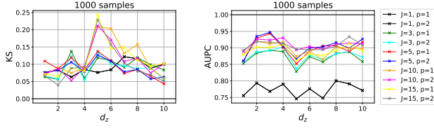
Figure 1. Comparison of the KS statistic (left) and the AUPC (right) of our test statistic \widehat{\text{NCI}}_{n,r,p} when the data is generated respectively from the models defined in (4) and (5) with Gaussian noises for multiple p and J . For each problem, we draw n = 1000 samples and repeat the experiment 100 times. We set r = 1000 and report the results obtained when varying the dimension d_z of each problem from 1 to 10. Observe that when J = 1 , for all p \geq 1 \widehat{\text{NCI}}_{n,r,1} = \widehat{\text{NCI}}_{n,r,p} , therefore there is only one common black curve.
