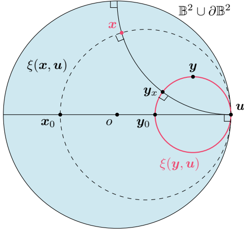
Figure 2: Poincaré disk \mathbb{B}^2 , boundary \partial\mathbb{B}^2 , point x (magenta), horosphere \xi(y, u) (magenta) through point y tangent to the boundary at u , and two geodesics (solid black) orthogonal to the boundary at u through o and x respectively. The signed composite distance \langle y, u \rangle from the origin o to the horosphere \xi(y, u) can be visualized as the Riemannian distance from o to point y_0 . Similarly, the distance between point x and horosphere \xi(y, u) is understood as the Riemannian distance between x and y_x along the geodesic, or equivalently, x_0 and y_0 .
