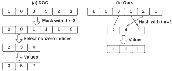
Figure 2. (a) The DGC algorithm for extracting top gradients and write it into the memory (b) DRAGONN. We overcome the overhead of nonzero indices selection by direct hashing.
