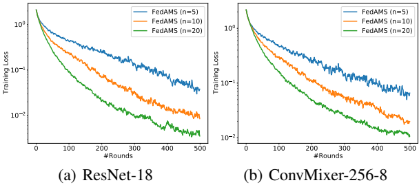
Figure 2. The learning curves for FedAMS with different participating number of clients n in training CIFAR-10 data on the ResNet-18 and the ConvMixer-256-8 models.
