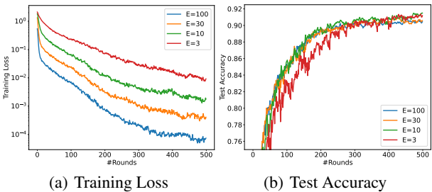
Figure 3. The learning curves for FedAMS with different number of local epochs E in training CIFAR-10 data on the ResNet-18 model.
