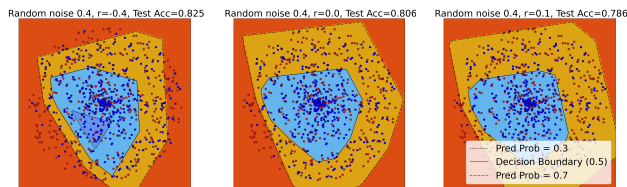
Figure 4. Model confidence visualization of NLS, VL, and LS on synthetic data (Type 1) with noise rate e_i = 0.4 . The optimal smooth rate is -0.4 . (left: NLS; middle: Vanilla Loss; right: LS). The test accuracy is annotated above each plot.
