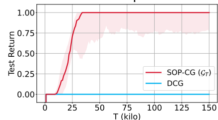
Figure 10. Extension of the illustrative example with 5 groups and each group 4 agents.
