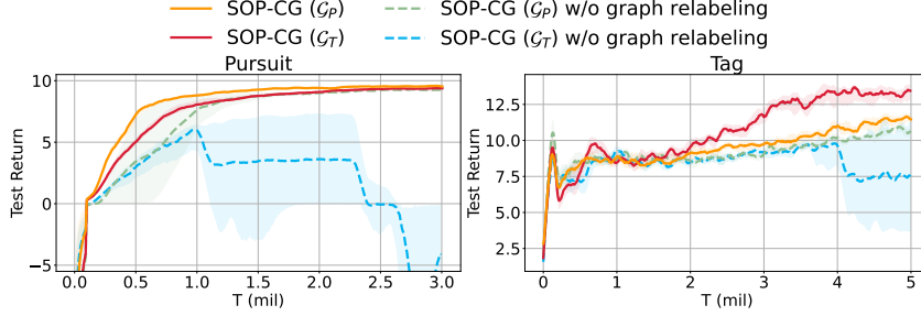
Figure 9. Ablation studies about the graph relabeling technique.
