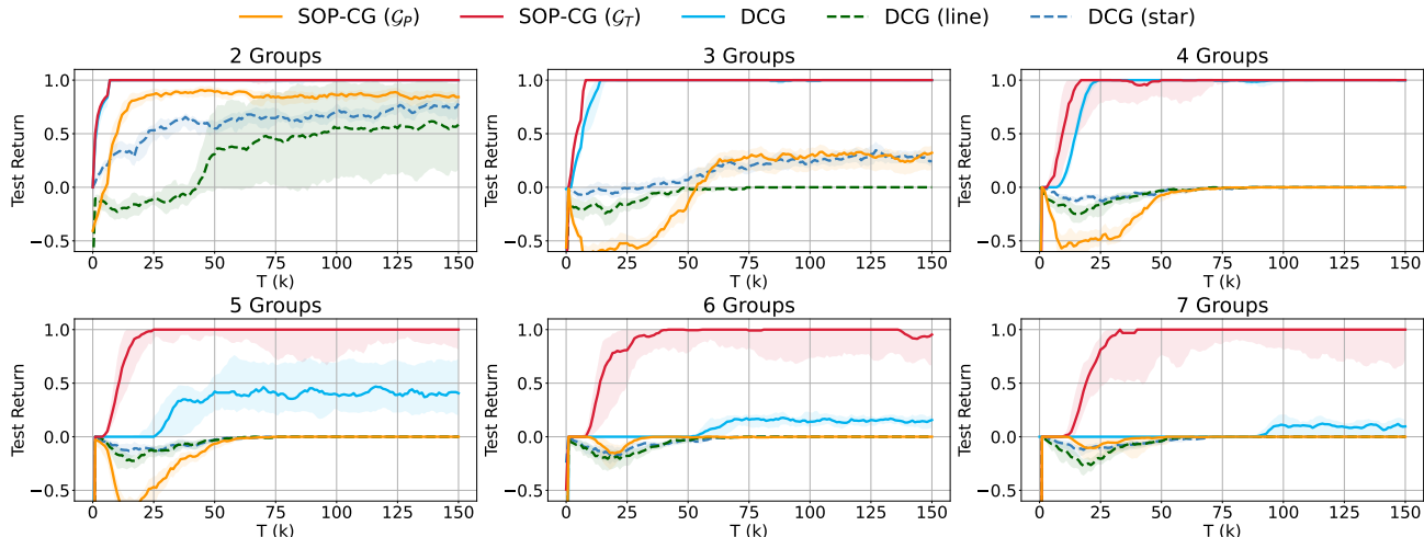
Figure 11. Learning curves on the illustrative example.
