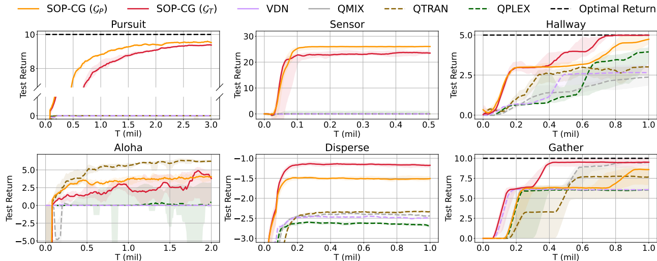
Figure 12. Comparison to fully decomposed value-based methods on MACO.
