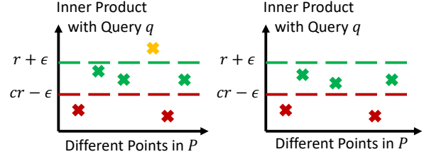
Figure 1: For query q , if there exists p^* \in P that has inner product \langle p, q \rangle \geq r + \epsilon (i.e., the yellow point), then the algorithm should return a point p \in P with \langle q, p \rangle \geq cr - \epsilon (i.e. green or yellow points in the left figure). Otherwise, no point needs to be returned (i.e., no point needs to be returned for the right-hand side figure).
