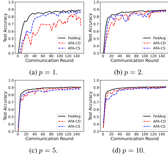
Figure 1. Test accuracy for logistic regression on non-i.i.d. MNIST with different p -values.
