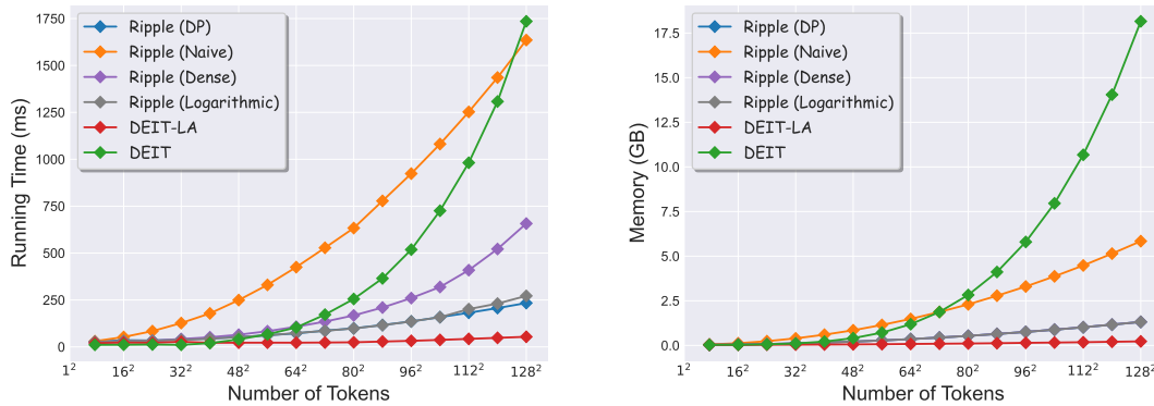
Figure 4: Empirical running time (left) and memory consumption (right) under different numbers of tokens, averaged by 5 runs.
