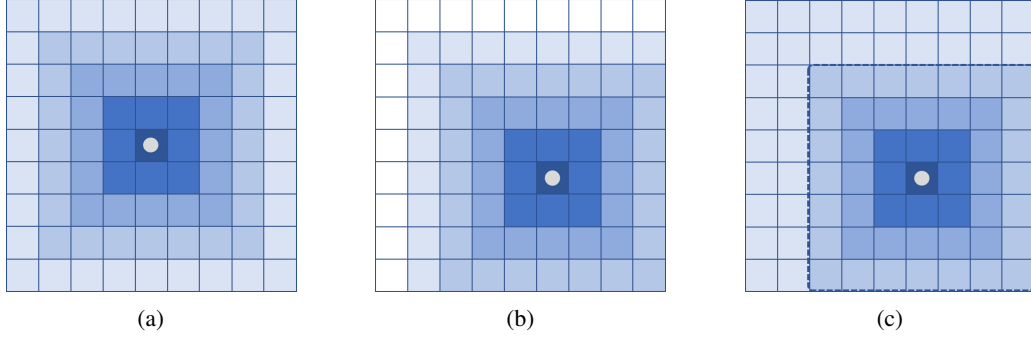
Figure 1: A demonstration of vicinal groups in ripple attention on a 9 \times 9 image I . Each square denotes a token, the circle denotes the query position and we use deeper color to indicate a larger spatial weight. Left (a) : an example of vicinal group partitioning in the case where the query lies in the center of an image, resulting in a symmetric rippling effect over the 2D space; Middle (b) : another group partitioning on the same image but the query token is not centered. In this case, distal vicinal groups (the top-left corner) receives almost no spatial weights. Right (c) : the same case as in (b) with the threshold \tau set such that \hat{r} = 4 . Groups beyond \hat{r} - 1 (indicated by the dashed line) contribute according to an equal spatial weight.
