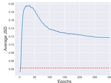
Figure 3: Training dynamic of average JSD between induced distributions of the proposed stick-breaking transform (SBT) and fixed exponentially decayed weights. The solid blue line denotes the training dynamic of JSD between SBT and FIXED-RIPPLE, while the dashed red line denotes the JSD between the uniform distribution and FIXED-RIPPLE.
