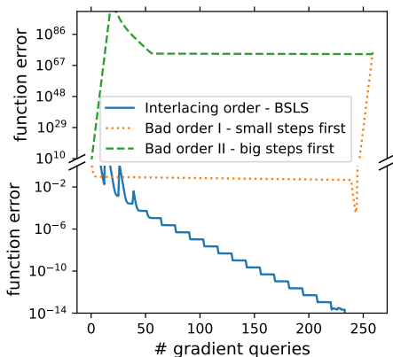
Figure 3: Importance of interlacing order in BLS under finite-precision arithmetic. Our objective is f(\mathbf{x}) = \frac{1}{2}\mathbf{x}^\top \mathbf{A}\mathbf{x} - \mathbf{b}^\top \mathbf{x} , where \mathbf{A} has eigenvalues in [0.001, 0.002] \cup [0.5, 1] . We consider three different step-size orderings, each running 20 big steps and 240 little steps in total. The first (solid) line runs BLS 1 (Algorithm 1), namely every big step is followed by 12 little steps. The second (dotted) line runs all little steps before the big steps. The third (dashed) line runs all big steps before the little steps. Observe that only the principled BLS converges under finite arithmetic (double-precision floating point format).
