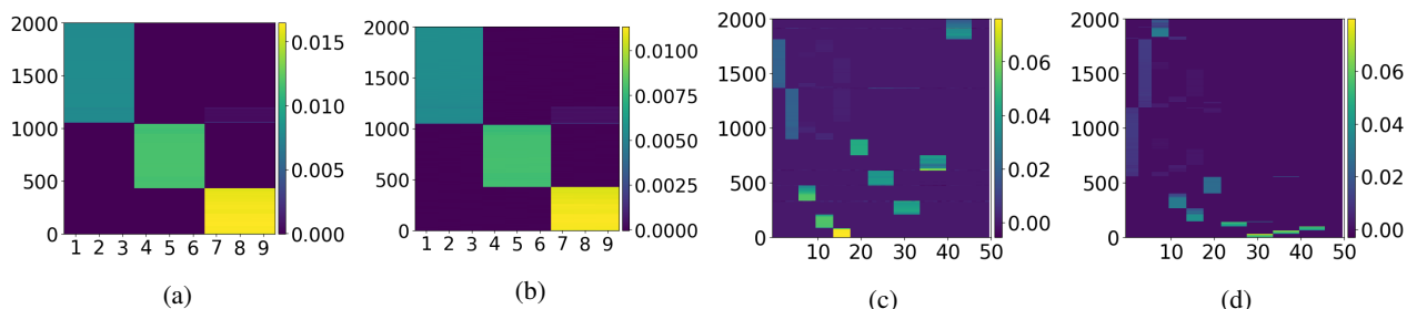
Figure 11: (a) Learning f_1^* using convex network with learnable c and 250 train samples. (b) Learning f_1^* using convex network with fix c to -1 and 250 train samples. (c) Learning f_4^* using convex network with learnable c and 30,000 train samples. (d) Learning f_4^* using convex network with fix c to -1 and 30,000 train samples.
