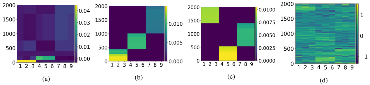
Figure 6: (a-c) Effect of training size on the learned model (see Learned models for different training sizes in the text) for the ground-truth model f_1^* . Panels a-c correspond to training sizes 800, 1500 and 7500. (d) Result for training on 7500 with large initialization.
