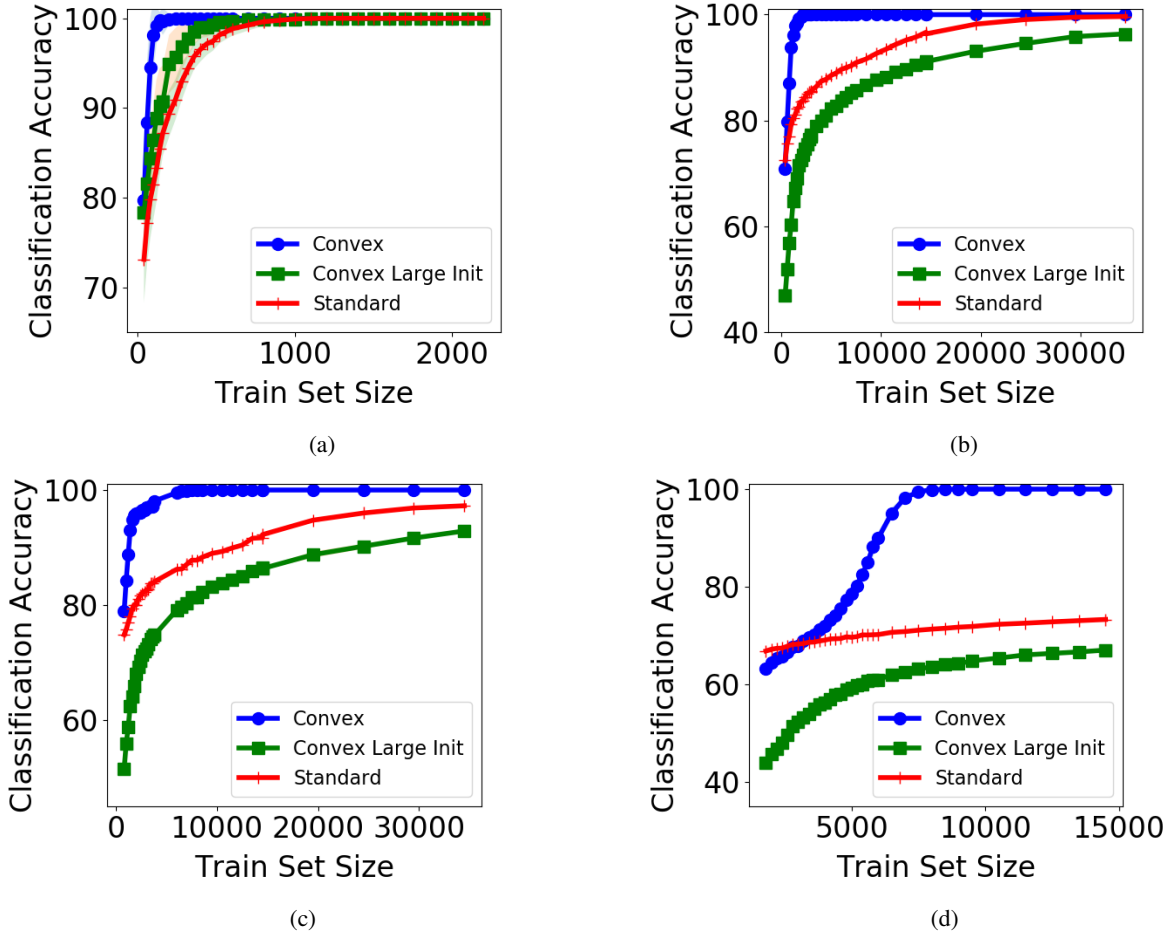
Figure 5: Test accuracy for the convex network with small initialization, convex network with large initialization and standard networks. Figure (a) shows the performance when learning f_1^* , Figure (b) for f_3^* , Figure (c) for f_4^* and Figure (d) for f_3^* (Results for f_2^* were presented in the main paper).
