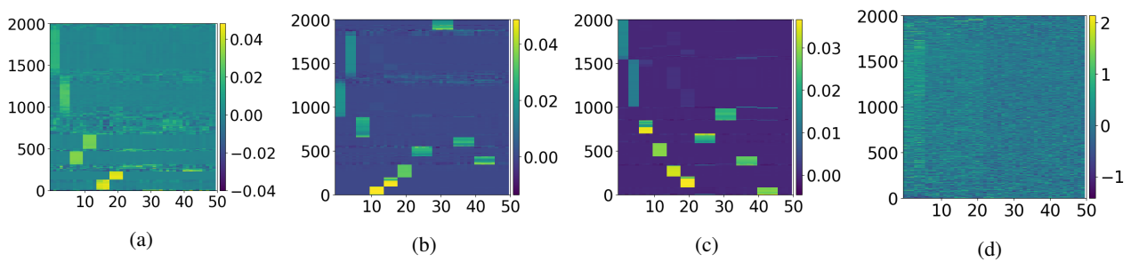
Figure 9: Same as Figure 6 but with f_4^* as ground truth.
