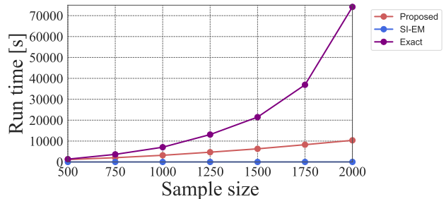
Figure 2: Run time comparison among proposed method (red), SI-EM (blue), and Exact (purple) on LinMean dataset with sample sizes n = 500, 750, \dots, 2000
