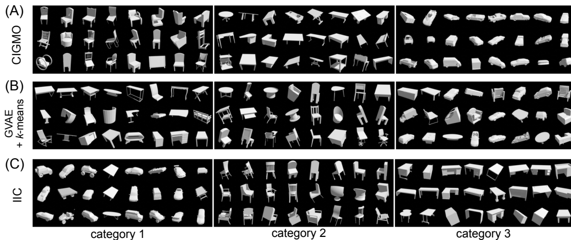
Figure 2: Examples of invariant clustering from (A) CIGMO, (B) GVAE [Hosoya, 2019] with k -means, and (C) IIC [Ji et al., 2019], for ShapeNet, in the case of 3 categories. Random 24 test images belonging to each estimated category are shown in a box. Note that the categories almost perfectly correspond to the chair, table, car image classes in (A). Such correspondence is much less clear in (B) and (C); in particular, cars are mixed with many other objects (category 3 in (B) and category 1 in (C)).
