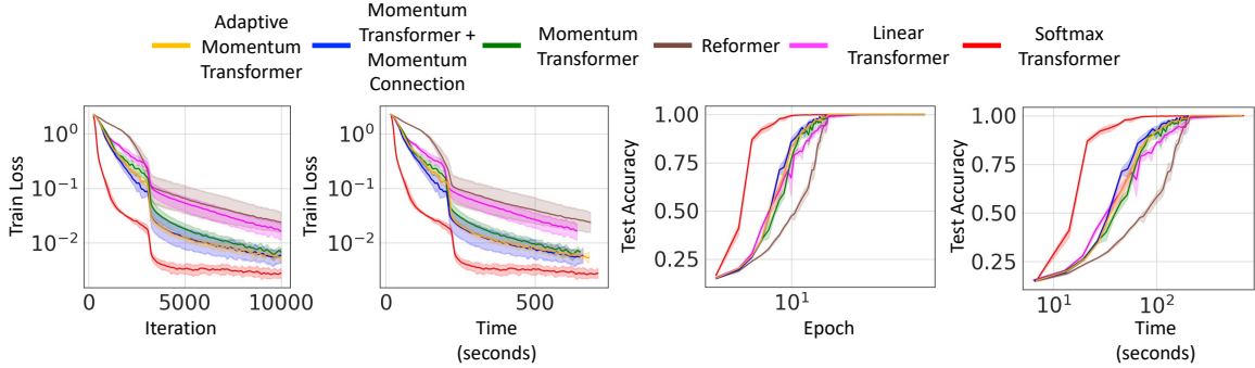
Figure 1: Convergence comparison of adaptive momentum, momentum, reformer, linear, and softmax transformer on the sequence copy task. Momentum and adaptive momentum transformers converge faster and achieve better training loss than both linear transformer and reformer. Softmax transformer converges the fastest but suffers from quadratic memory and computational complexities. Adaptive momentum transformer performs as well as momentum transformer without intensively searching for momentum values. The training time per epoch for softmax transformer, reformer, linear transformer, our momentum transformer without and with momentum connection, and our adaptive momentum transformer are 7.1, 6.9, 6.4, 6.5, 6.6, and 6.8 seconds, respectively. Here, the computational time per epoch does not reveal a significant advantage of efficient transformers over the softmax transformer because the sequence length is only 128.
