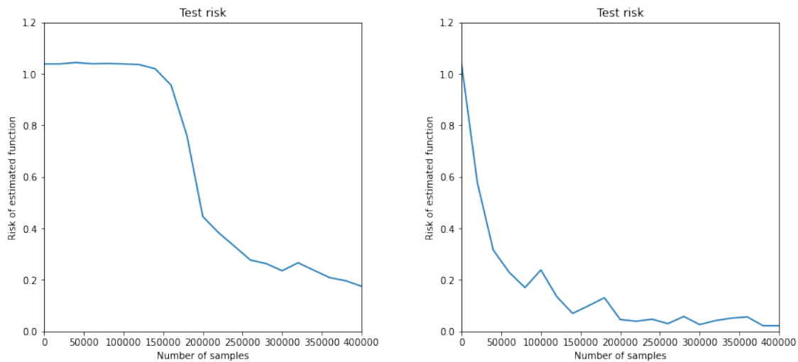
(a) Leap-3 function h_*(z) = \text{He}_3(z_1)
