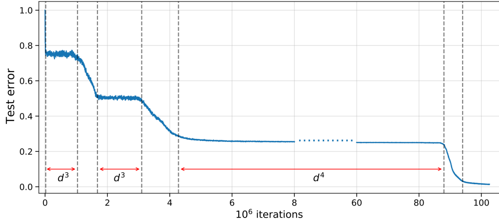
Figure 1: Test error versus the number of online-SGD steps to learn h_*(z) = z_1 + z_1 z_2 \cdots z_5 + z_1 z_2 \cdots z_9 + z_1 z_2 \cdots z_{14} in ambient dimension d = 100 on the hypercube. We take M = 300 neurons with shifted sigmoid activation and train both layers at once with constant step size 0.4/d . The SGD dynamics follows a saddle-to-saddle dynamic and sequentially picks up the support and monomials z_1 in roughly d steps, z_1 z_2 \cdots z_5 in d^3 steps (leap of size 4), z_1 z_2 \cdots z_9 in d^3 steps (leap of size 4) and z_1 z_2 \cdots z_{14} in d^4 steps (leap of size 5).
