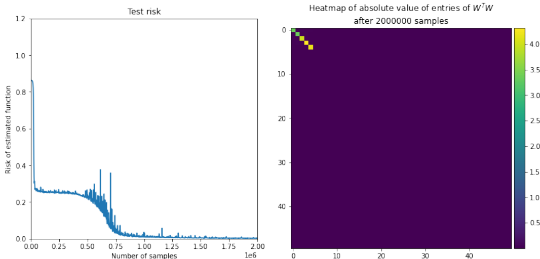
Figure 2: In this figure we consider training a 5-layer ResNet with fully-connected layers with SGD the leap-3 function h_*(z) = 2 \cdot \prod_{i=1}^2 \tanh(z_i) + 5 \cdot \prod_{i=1}^5 \tanh(z_i) with data \mathbf{x} \sim \mathcal{N}(0, I_d) and d = 50 . While our paper considered bounded degree polynomials, the leap complexity, which drives the sequential alignment to the support, also holds for non-polynomial functions. In this case, the leap depends on the first non-zero monomials in the Hermite decomposition. For h_* considered in this plot, we have first a leap of size 2 to align with x_1, x_2 followed by a leap of size 3 to align with x_3, x_4, x_5 . In the plot of test risk over time, we indeed see first a short saddle to align with x_1, x_2 , followed by a quick decrease of the loss (corresponding to the neural networks fitting 2 \tanh(z_1) \tanh(z_2) ). This is followed by a plateau while SGD slowly picks up x_3, x_4, x_5 (saddle) and a sharp decrease in the loss when the neural network fit the remainder of h_* . We also plot the heatmap of the absolute value of the entries of \mathbf{W}^T \mathbf{W} \in \mathbb{R}^{d \times d} where \mathbf{W} is the first-layer matrix after training. This shows that the first layer indeed picks up the relevant coordinates (first 5 coordinates) in the support after training.
