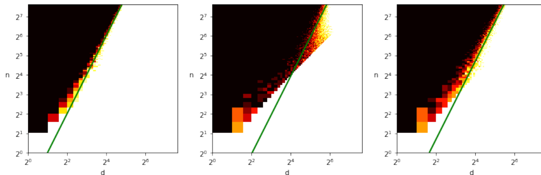
Figure 18: Plots from Figure 1 on a \log_2 scale. (Left) Ellipsoid fitting SDP, (Middle) : Least-squares, (Right) : Identity perturbation
