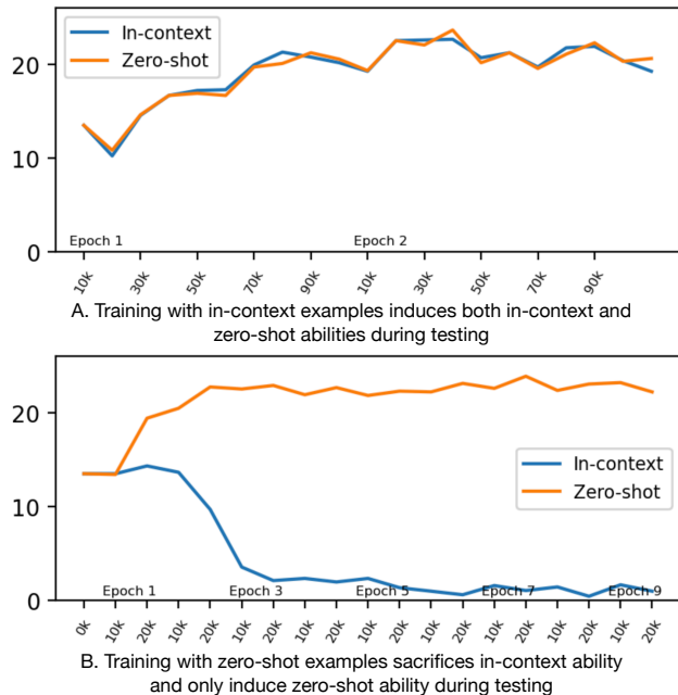
Figure 4. X-axis means tuning datapoints, y-axis means validation accuracy on GSM8K. Both figures use FlanT5 3B as the base model. A : training with in-context examples automatically give the model zero-shot ability. B : training with zero-shot examples sacrifices in-context ability.
