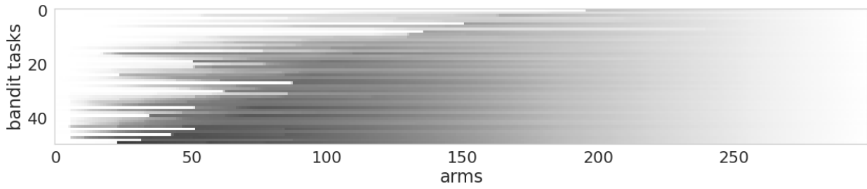
(b) 50 mean reward vectors generated by the diffusion model trained on perfect data.
