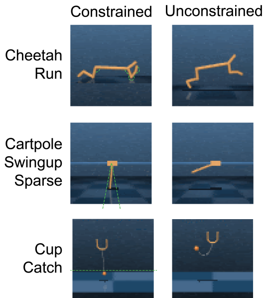
Figure A12. Constrained Control Suite tasks. Green dashed lines represent the constraints. For cup, the z-range of the ball was limited to [-.151 \text{ } -.091] . For cartpole, the hinge of the pole was limited to angles [175 \text{ } 185] . For cheetah, the limits of the joints were b\text{thigh} [50 \text{ } 60] , f\text{thigh} [-57 \text{ } -52] , f\text{shin} [-70 \text{ } -60] , f\text{foot} [-28 \text{ } -26] . In all cases, at T_0 = 500K , all constraints were released.
