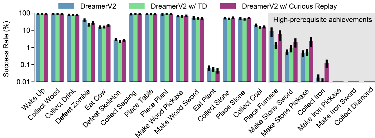
Figure A15. DreamerV2 agent ability spectrum showing the success rates for supervised Crafter, ordered from left to right by number of prerequisites for an achievement (n=8 each condition, mean ± s.e.m.). Curious Replay succeeds at challenging achievements that are unlocked only by many prerequisite. Highlighted high-prerequisite achievements need at least four preceding achievements.
