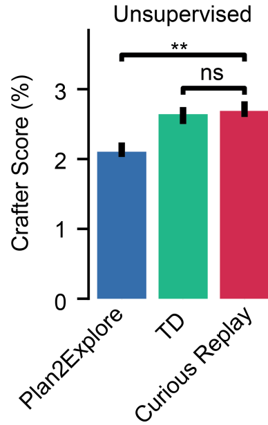
Figure A14. Score on the unsupervised (no extrinsic reward) version of Crafter (n=8 each condition, mean +/- s.e.m., independent t-test with fdr-bh correction).
