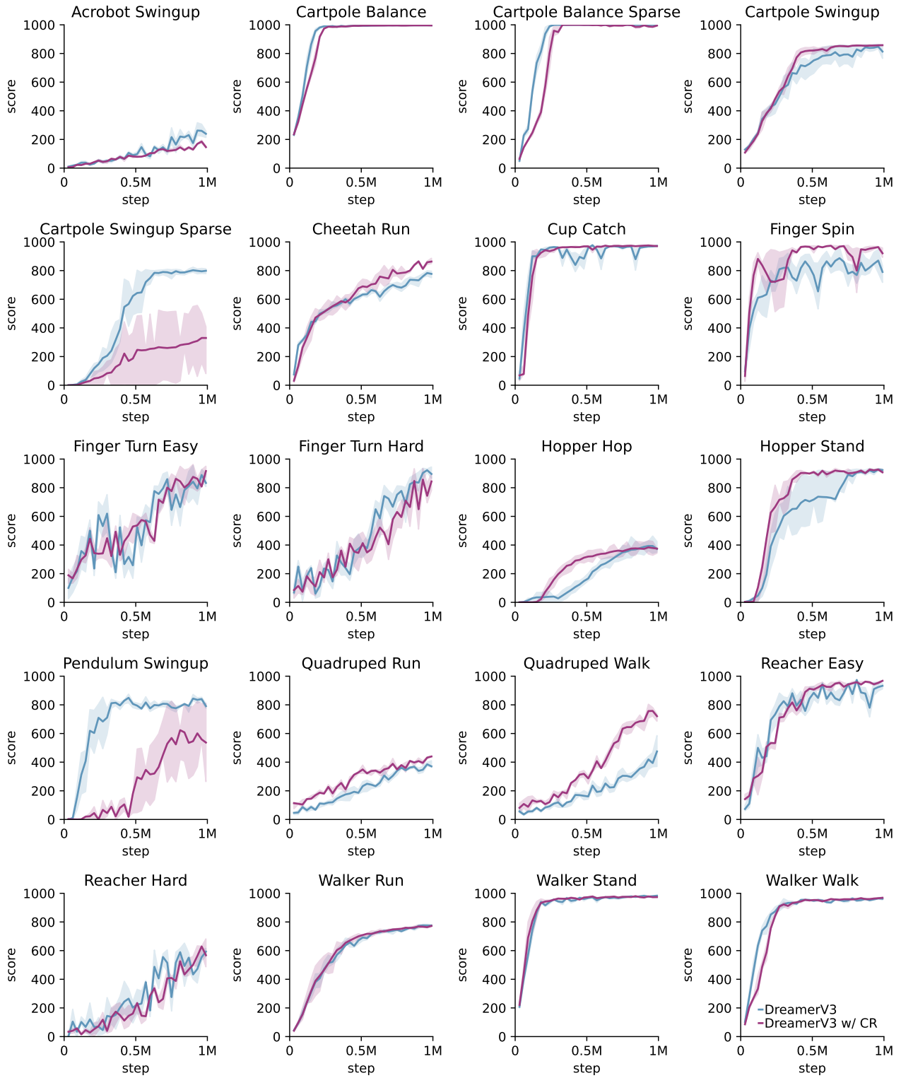
Figure A19. Deepmind Control Suite, comparing DreamerV3 and DreamerV3 with Curious Replay. Curious Replay improves performance on tasks such as Quadruped Walk, while decreasing performance on tasks such as Cartpole Swingup Sparse (n=3 per task, mean \pm s.e.m.).
