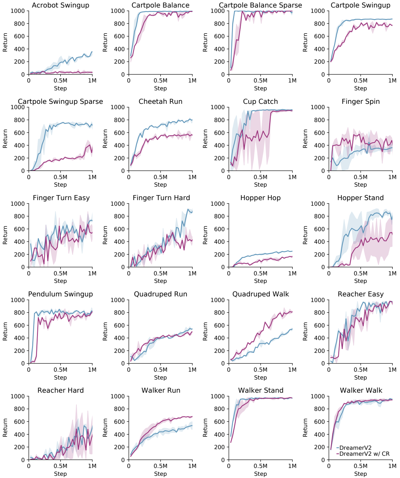
Figure A18. Deepmind Control Suite, comparing DreamerV2 and DreamerV2 with Curious Replay. Curious Replay improves performance on tasks such as Quadruped Walk and Walker Run, while decreasing performance on tasks such as Acrobot Swingup and Cartpole Swingup Sparse (n=2 per task, mean \pm s.e.m.).
