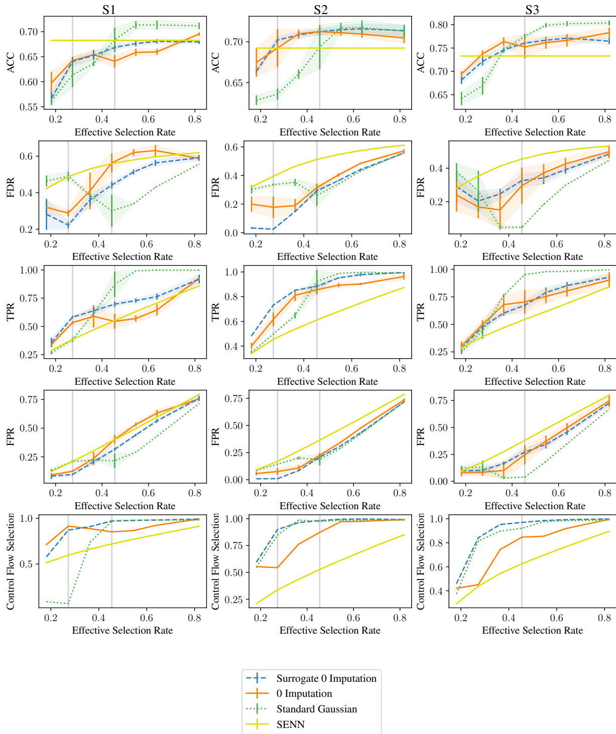
Figure 10: Performances of LEX with different imputations. 0 imputation (solid orange line) corresponds to the imputation method of InvasE/L2X, Surrogate 0 imputation (blue dashed line) is the imputation method of REAL-X. The standard Gaussian is the true conditional imputation method from the model (green dotted curve). We also conducted experiments on self-explainable neural networks (SENN) in dark continuous green. The columns correspond to the three synthetic datasets (S1, S2, S3) and the lines correspond to the different measure of quality of the model (Accuracy, FDR, TPR and control flow selection). We report the mean and the standard deviation over 5 folds/generated datasets.
