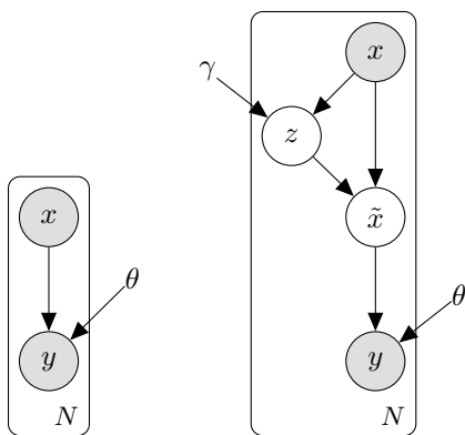
Figure 1: The LEX pipeline allows us to transform any prediction model into an explainable one. In supervised learning, a standard approach uses a function f_\theta (usually a neural network) to parameterize a prediction distribution p_\theta . In that framework, we would feed the input data directly to the neural network f_\theta . Within the LEX pipeline, we obtain a distribution of masks p_\gamma parameterized by a neural network g_\gamma from the input data. Samples from this mask distribution are applied to the original image x to produce incomplete samples x_z . We implicitly remove features by sampling imputed samples \tilde{x} given the masked image using a generative model p_tilde conditioned on both the mask and the original image. These samples are then fed to a classifier f_\theta to obtain a prediction. As opposed to previous methods, multiple imputation allows us to minimise the encoding happening in the mask and to get a more faithful selection.
