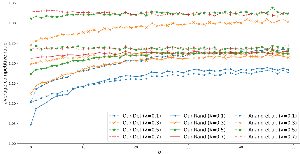
Figure 2. Average competitive ratio achieved by Our-Det (dashed line), Our-Rand (solid line), and Anand et al. (dotted line) are shown as a function of \sigma . Different colors/markers correspond to different values of the trade-off parameter \lambda .
