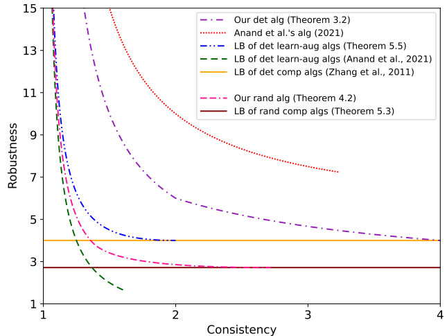
Figure 1. The consistency-robustness trade-off of learning-augmented algorithms.
