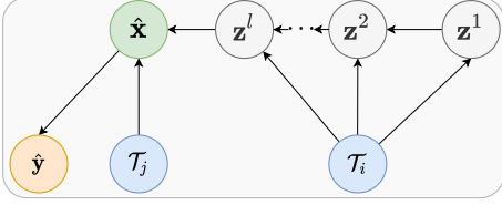
Figure 3. Hierarchical variational task modulation. \mathbf{z}^l indicates the latent modulation parameters at the layer l . The latent transformation parameter \mathbf{z}^l is dependent on the task \mathcal{T}_i and the upper \mathbf{z}^{l-1} .
