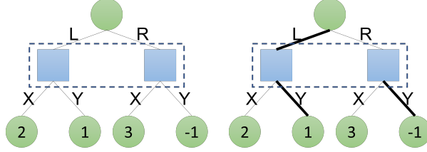
Figure 4. An example of two iterations of Extensive-form Double Oracle. Square player is unaware of what Circle player chose. The values at the leafs are Circle player’s payoff. Since it is zero-sum game, the Square player’s payoffs are the opposite numbers.
