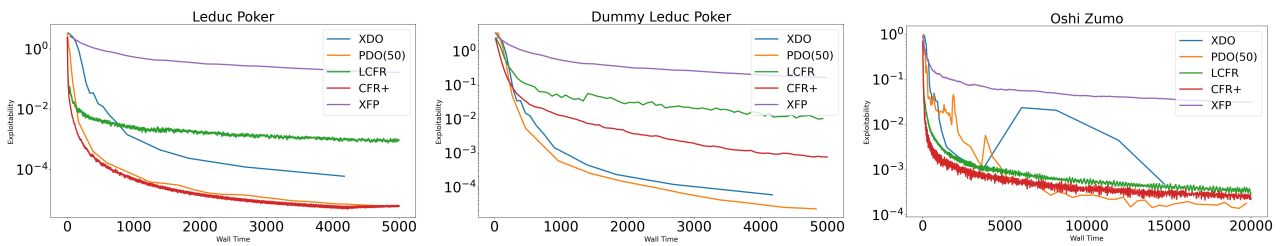
Figure 9. Performance of PDO with periodicity 50 and other baselines including Linear CFR (exploitability-wall time).
