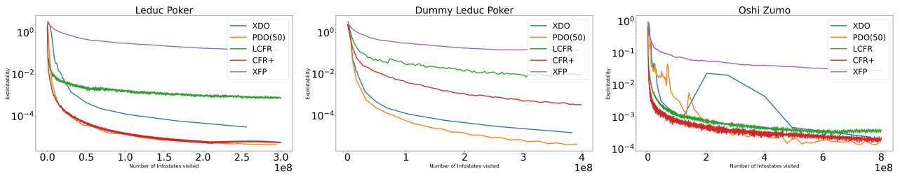
Figure 8. Performance of PDO with periodicity 50 and other baselines including Linear CFR (exploitability-number of infostates visited).
