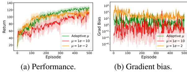
Figure 5. Barrier Smoothing applied to FOPG when equipped with different designs of the central-path parameter \mu .
