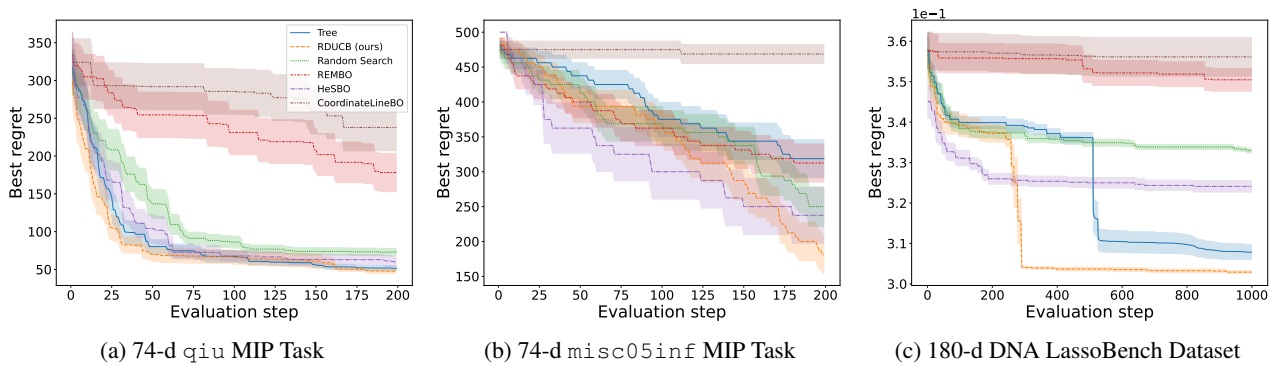
Figure 3. Best regret results from tuning 74-d MIP problems and the 180-dimensional DNA dataset from the Lasso bench. We average the results over 40 seeds for qiu and 80 seeds for misc05inf. For the LassoBench task, we average over ten random seeds. Tree again refers to the previous state-of-the-art from (Han et al., 2021). We see that RDUCB outperforms others in best regret. Interestingly, the performance gap to other methods increases as the dimensions increase.
