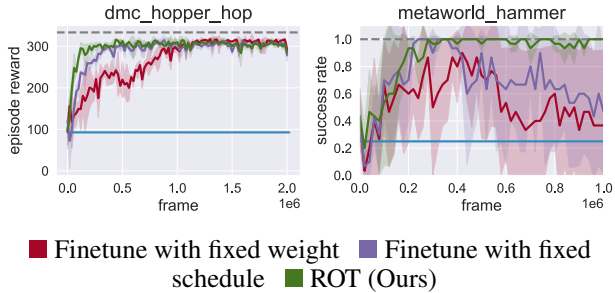
Figure 6: Effect of various BC regularization schemes compared with our adaptive soft-Q filtering regularization. We hypothesize this improvement is primarily due to the better stability of adaptive weighing as seen in the significantly smaller standard deviation on the Meta-world tasks.
