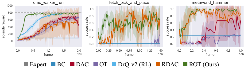
Figure 5: Ablation analysis on the choice of base IRL method. We find that although adversarial methods benefit from regularized BC, the gains seen are smaller compared to ROT. Here, we also see that ROT can outperform plain RL that requires explicit task-rewards.
