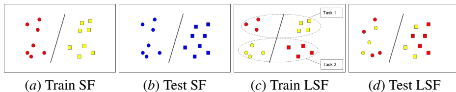
Figure 1: Spurious features and local spurious features. If the task is to distinguish the squares from the circles. In Fig. 1(a) and 1(b), the color is a spurious feature because there is a covariate shift between train and test data. In Fig. 1(c) and 1(d), we observe two tasks of a domain-incremental scenario, the colors are locally spurious in tasks 1 and 2. Even if there is no significant covariate shift between train and test full data distribution, colors appear discriminative while looking at data within a task.
