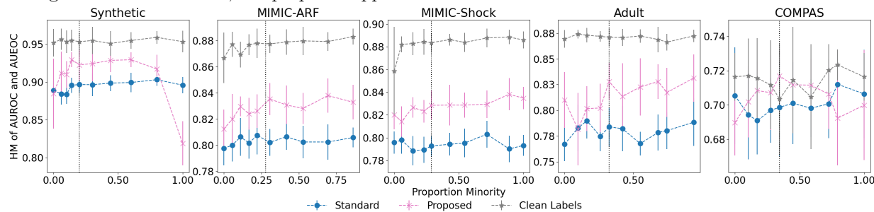
(b) We varied the alignment set bias (proportion of minority instances). The proposed approach is generally robust to variations in bias. The dashed vertical black line shows an unbiased alignment set.
