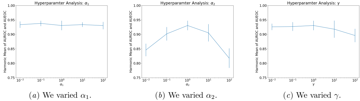
Figure 7: Sensitivity analysis of proposed approach on objective function hyperparameters.
