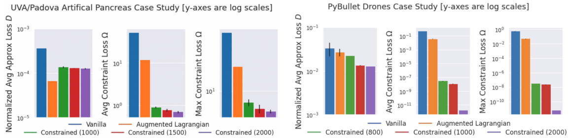
Figure 5: Bar charts of approximation loss on \mathcal{D} , average constraint loss on \Omega , and maximum constraint loss on \Omega (for 3 random seeds) after training completes for AP (left), and Drones (right). Plots of these metrics vs gradient steps for both case studies are in the Appendix of our complete version (Sridhar et al., 2022a).
