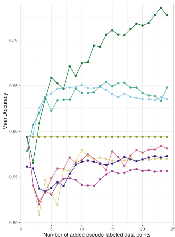
Figure 2: Results on Simulated Data. Legend: See Figure 1.
