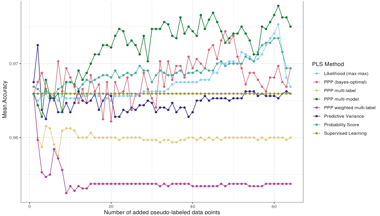
Figure 1: Results of Self-Training with Different PLS Methods on Banknote Data (One Instance Added per Iteration).
