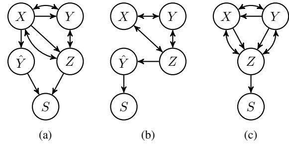
Figure 2: Causal graphs relating to examples of PMAR.
