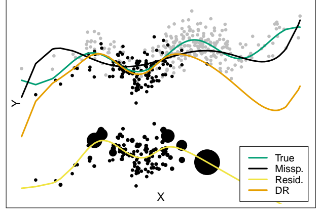
Figure 7: Doubly robust regression. At the top the (X, Y) pairs are plotted, with the true model (green) and misspecified RR model (black). The residuals of the misspecified model are plotted at the bottom. The IW regression model for the residuals (yellow) is then added to the misspecified model, which yields the doubly robust model (orange).
