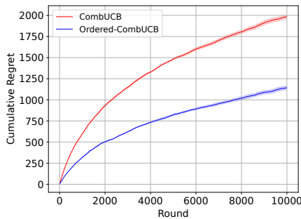
Figure 2: Comparison of cumulative regret for CombUCB and Ordered CombUCB on synthetic Bernoulli bandit instance.
