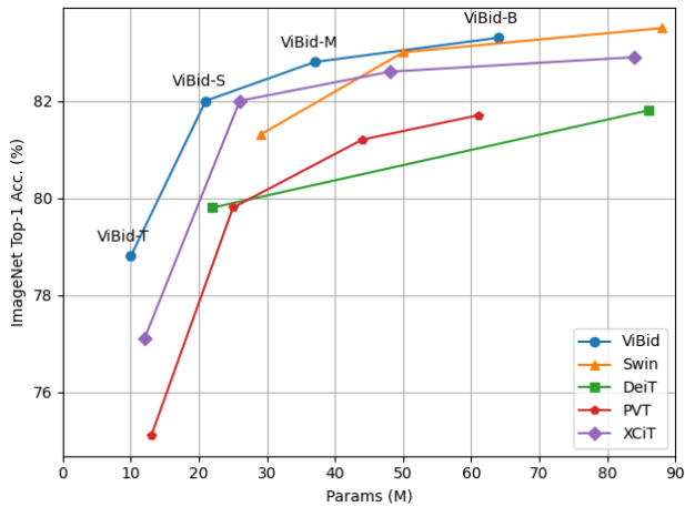
(b) Params vs. ImageNet Top-1 Acc.
