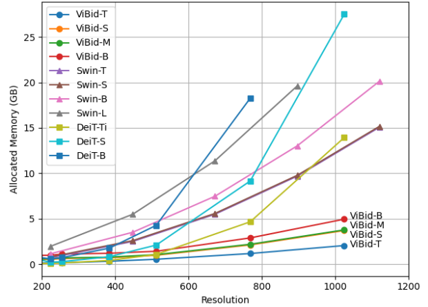
(a) Allocated memory according to the input resolution
