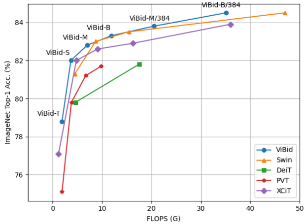
(a) FLOPs vs. ImageNet Top-1 Acc.
