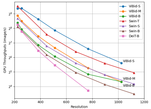
(b) GPU throughput according to the input resolution
