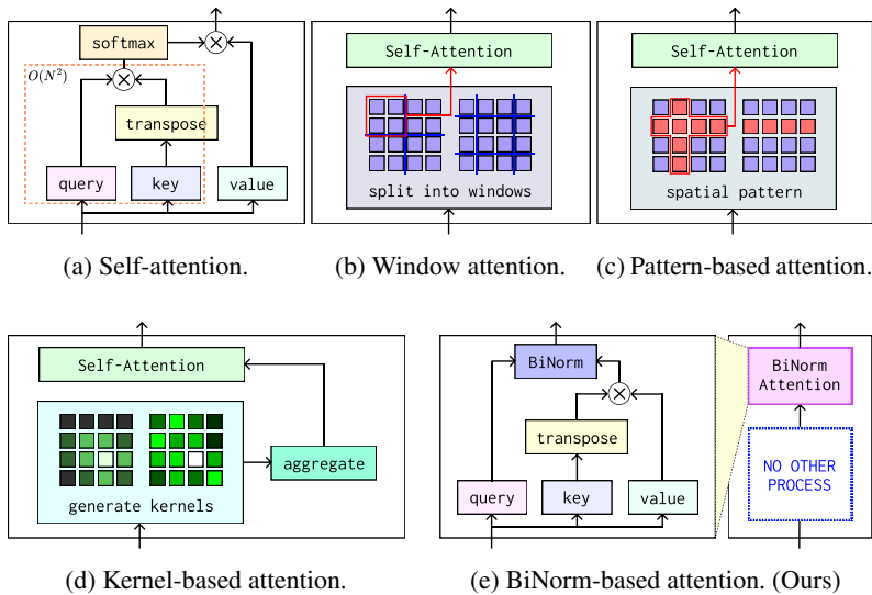
Figure 1: Comparison with existing self-attention algorithms: (a) Self-attention: The query and key generate N \times N attention maps, resulting in an O(N^2) operation. (b) Window attention: This method splits input images into several windows before computing self-attention. While it avoids the O(N^2) problem of self-attention, it also slows down computation due to a fixed window size. (c) (d) Efficient self-attention: These methods choose a fixed number of tokens to generate attention maps. However, these procedures are heuristic and complicated, and some of them require operations not supported by common frameworks. (e) Ours: BiNorm-based self-attention is not as complicated and has an O(N) complexity since it does not require any additional processing.
