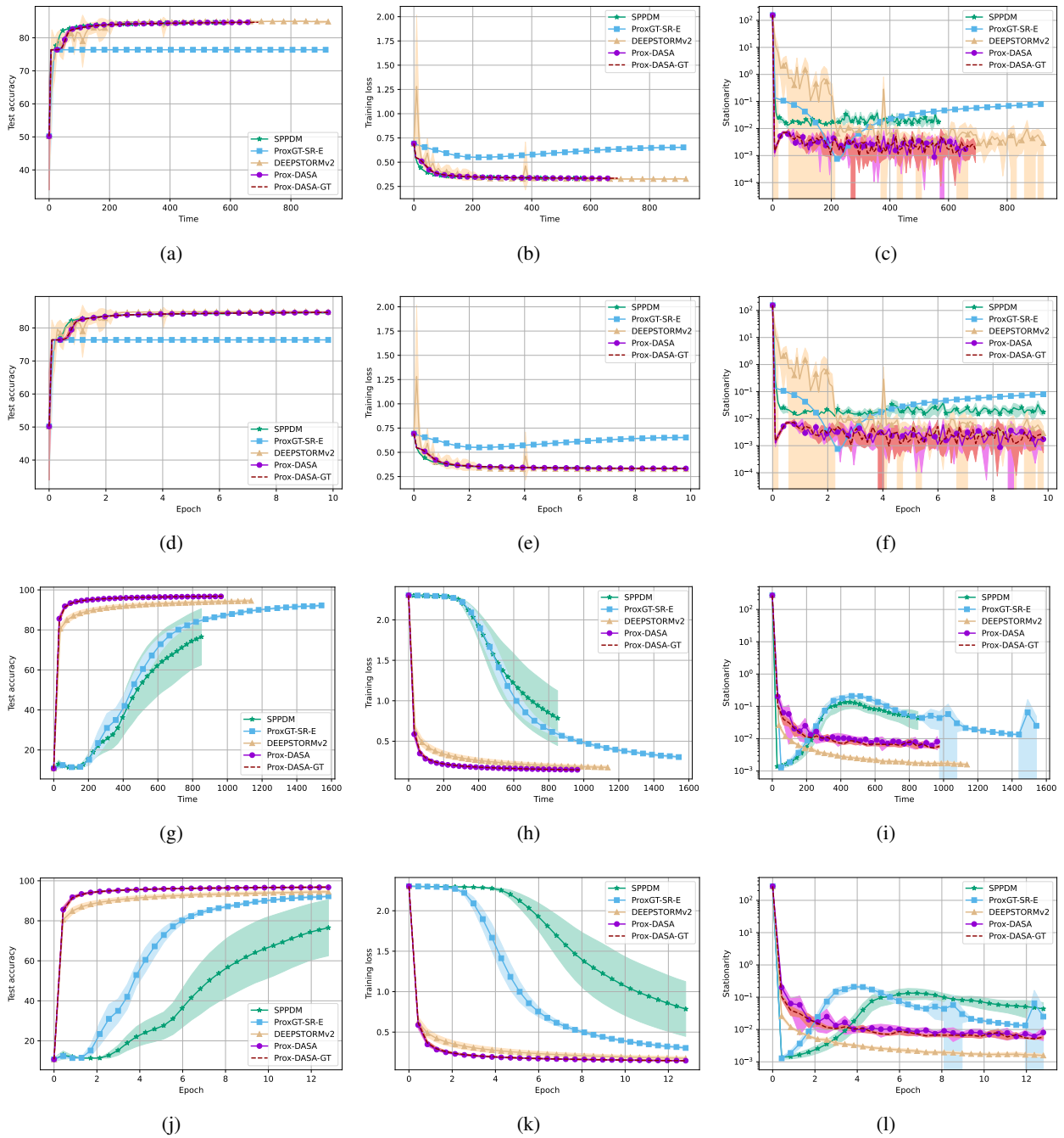
Figure 2: Comparisons between SPPDM [Wang et al., 2021], ProxGT-SR-E [Xin et al., 2021a], DEEPSTORM [Mancinoball et al., 2023], Prox-DASA 1, and Prox-DASA-GT 2. The first two rows correspond to a9a and the last two rows correspond to MNIST. The results are averaged over 10 trials, and the shaded regions represent confidence intervals. The vertical axes in the third column are log-scale. It should be noted that ProxGT-SR-E maintains another hyperparameter q (see, e.g., Algorithm 4 and Theorem 3 in [Xin et al., 2021a]) and computes gradients using a full batch every q iterations. For simplicity, we do not include that amount of epochs when we plot this figure. In other words, the real number of epochs required to obtain a point on ProxGT-SR is larger than plotted in the figures in the second and fourth rows. We include the plots that take q into account in Appendix.
