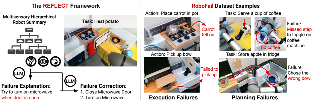
Fig 1: A framework for robot failure explanation and correction. On the left, we show the REFLECT framework that converts multisensory observations (RGB-D, audio, robot states) to a hierarchical summary of robot experiences. The summary is then used to query a Large Language Model (LLM) for failure explanation and correction. The right shows a few example failure cases in the RoboFail dataset.
