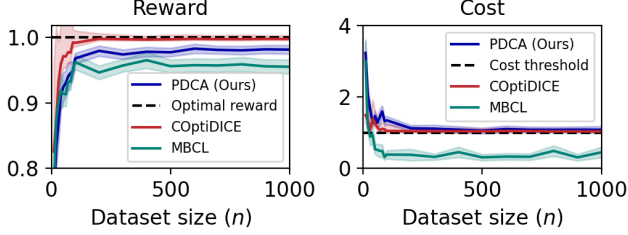
Figure 1: Tabular CMDP experiment
