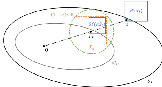
Figure 1: Graphical representation of the approach for lower bounding \gamma_t (in ROFUL) for the setting with linked convex constraints.
