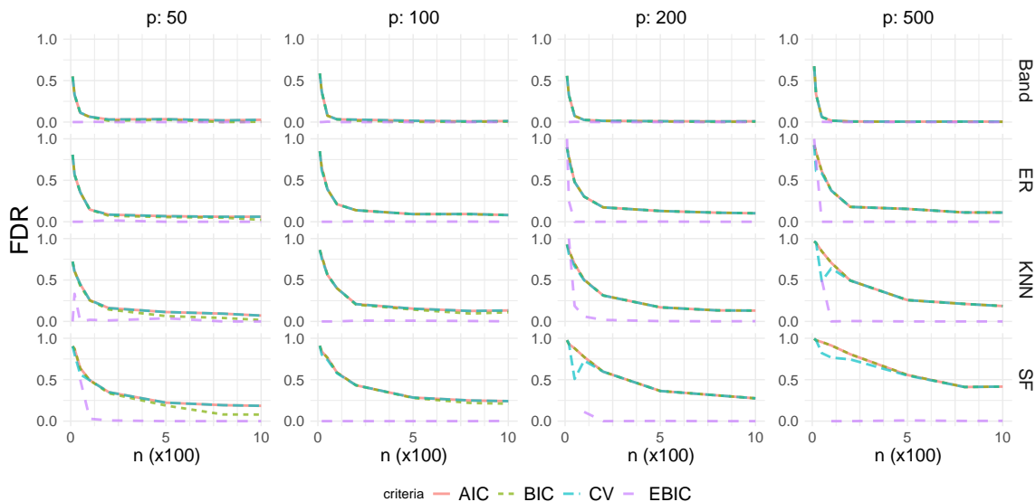
Figure 5: FDR vs. sample size n (in hundreds) and p on different graph types with NS to compare criteria.
