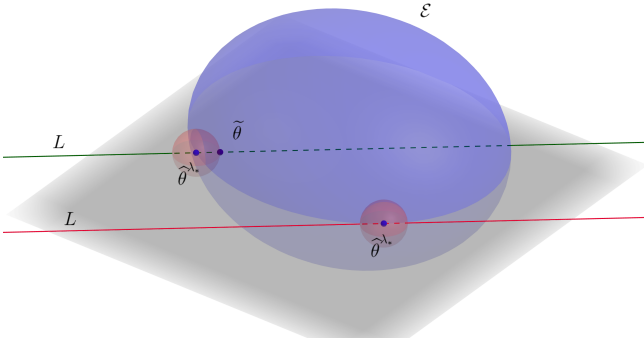
Figure 1: Illustration of the ellipsoid \mathcal{E} and the line L when p - 1 = 3 and \widehat{\mathbf{n}}\mathbf{e}^{\lambda^*} = \widehat{\mathbf{n}}\mathbf{e}^G = \{1, 2\} . (green) There exists another Lasso solution \tilde{\theta} inside \mathcal{E} when it is not a tangent line. (red) No Lasso solution can be found inside \mathcal{E} when it is a tangent line.
