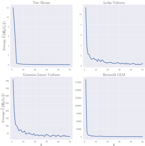
Figure 2: Average volume estimates \hat{\ell}(\{\mathcal{B}_{\hat{q}}(\hat{c}_k^{(i)})\}) over x^{(i)} \in \mathcal{D}_{\mathcal{C}_2} across SBI benchmarks.
