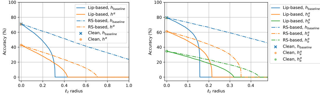
(b) h_{\text{baseline}}(\cdot) : RS with \sigma = 0.25 . Consider two mixed classifier examples: h_a^\alpha(\cdot) : \alpha = 0.76 ; h_a(\cdot) is RS with \sigma = 0.5 ; h_b^\alpha(\cdot) : \alpha = 0.67 ; h_b(\cdot) is RS with \sigma = 1.0 .
