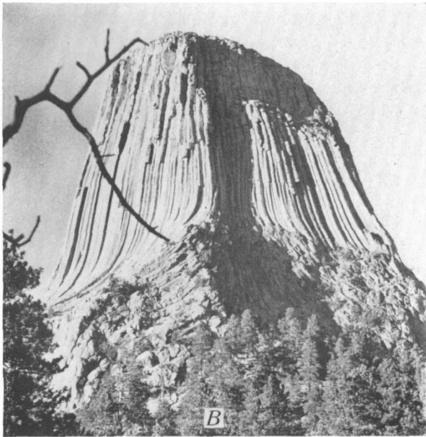
FIGURE 53.— A . Northwest side of Devils Tower showing how the columns taper or converge and in places unite near the top and are cut by numerous cross-fractures. B . South side of Devils Tower showing the columns flaring out and merging to form the massive base.
