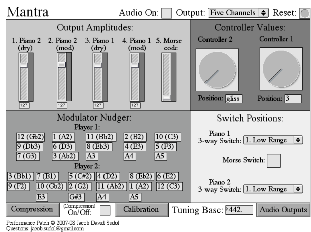
Figure 2. Max/MSP interface for Mantra displays the positions for each performer's controller and switches as well as levels and other features that can be controlled by the sound projectionist.
